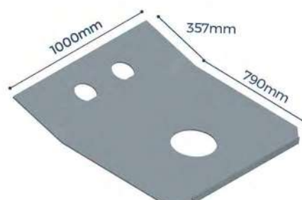
FR0604 MESA PINO REI CHAPA 7,94mm
