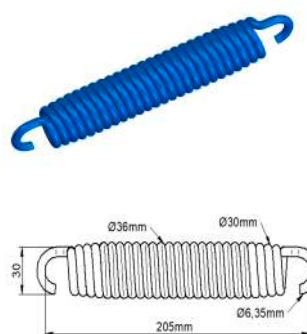
Mola Patimtraseiro Volvo N10/N12 B10B/B10L/B10M/B10R/B12/B12M/ B58/B12M/B7/B7L/B7R/F10/F12/ N10Usa/N12Usa/Ni10/Ni12
