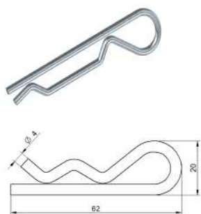
Grampo "R" (4X62mm) F4059B - zincado branco
