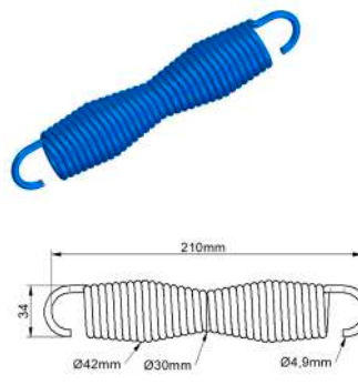
Mola Patim de Freio Dianteiro - Volvo B10B/B10L/B10M/B10R/B12/B12M/ B58/B12M/B7/B7L/B7R/F10/F12/ N10Usa/N12Usa/Ni10/Ni12
