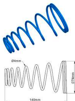
Mola Sprin Brake 16X24/20X30/24X30/30X30
