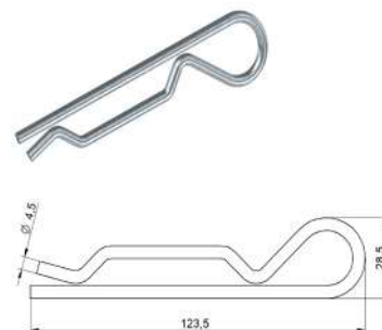
Grampo "R" (4,5X123,5mm) F4059 - zincado branco
